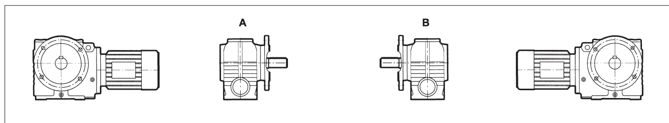
Output Shaft Position
