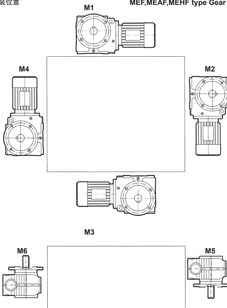
MEF,MEAF,MEHF type Gear Unit Mounting Position
